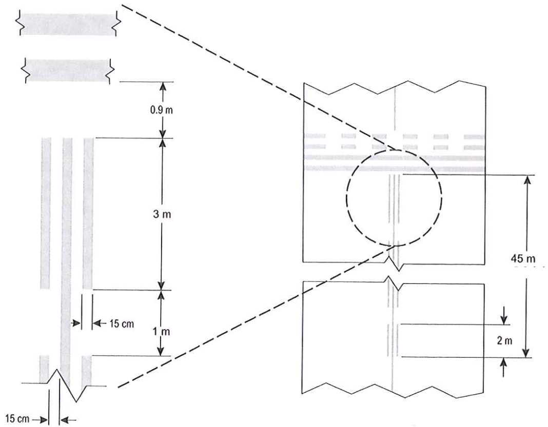
Figure 1: Enhanced Taxiway Centre Line Marking
