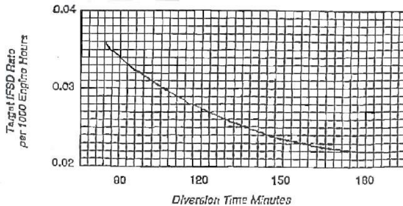
Figure 1: Target IFSD Rate versus Diversion Time
